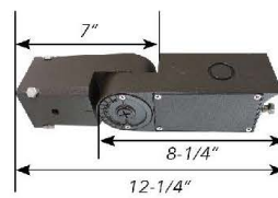
LF3-SF Adjustable slip fitter for pole mount 2"-2 1/2" with K/O to install PC or sensor (LF3-80, 100, 150, 220 & 300)
