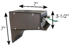
LF3-EXTARM Straight extension arm for shoe box application, with K/O to install PC or sensor (LF3-80, 100, 150, 220 & 300)
